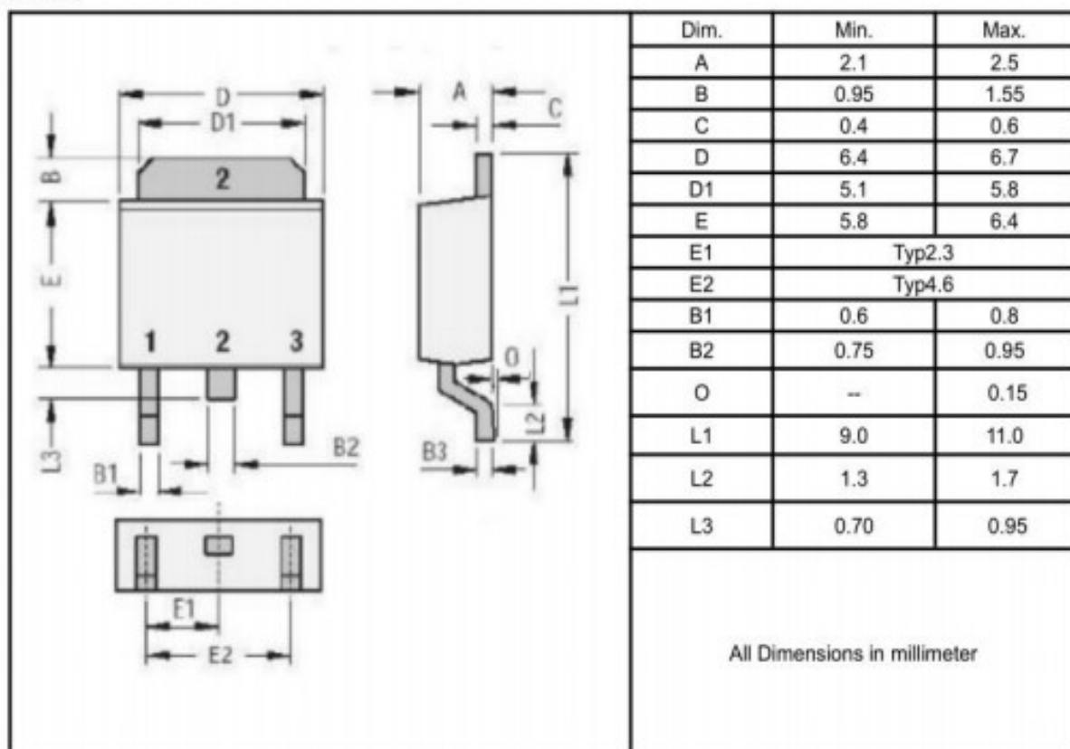
TO-252
