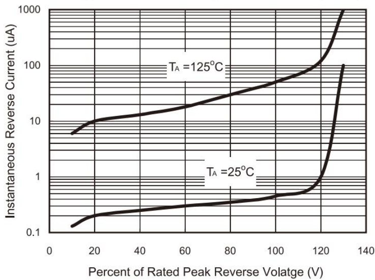
FIG 3 Typical Reverse Leakage Characteristics per Leg
