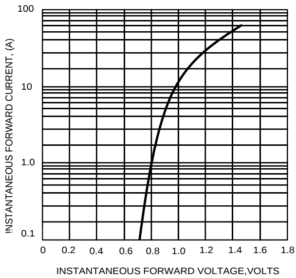
FIG.3-TYPICAL FORWARD CHARACTERISTICS
