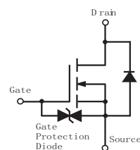
■ Simplified outline(SOT-323)
